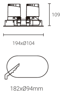
Fixed Fixture
